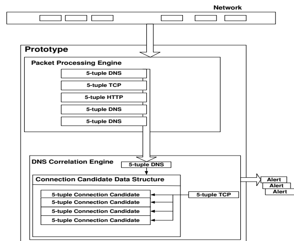
Figure 3. High-level System Design
