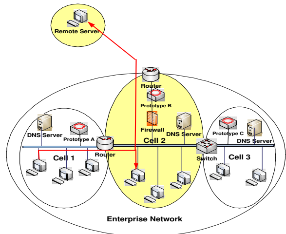
Figure 2. DNS Anomaly-based Detection Deployment
